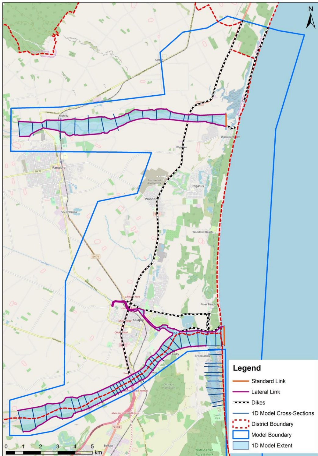
Figure 6: Model schematisation
